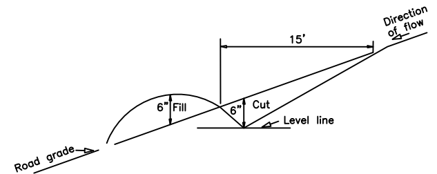
WATER BAR
