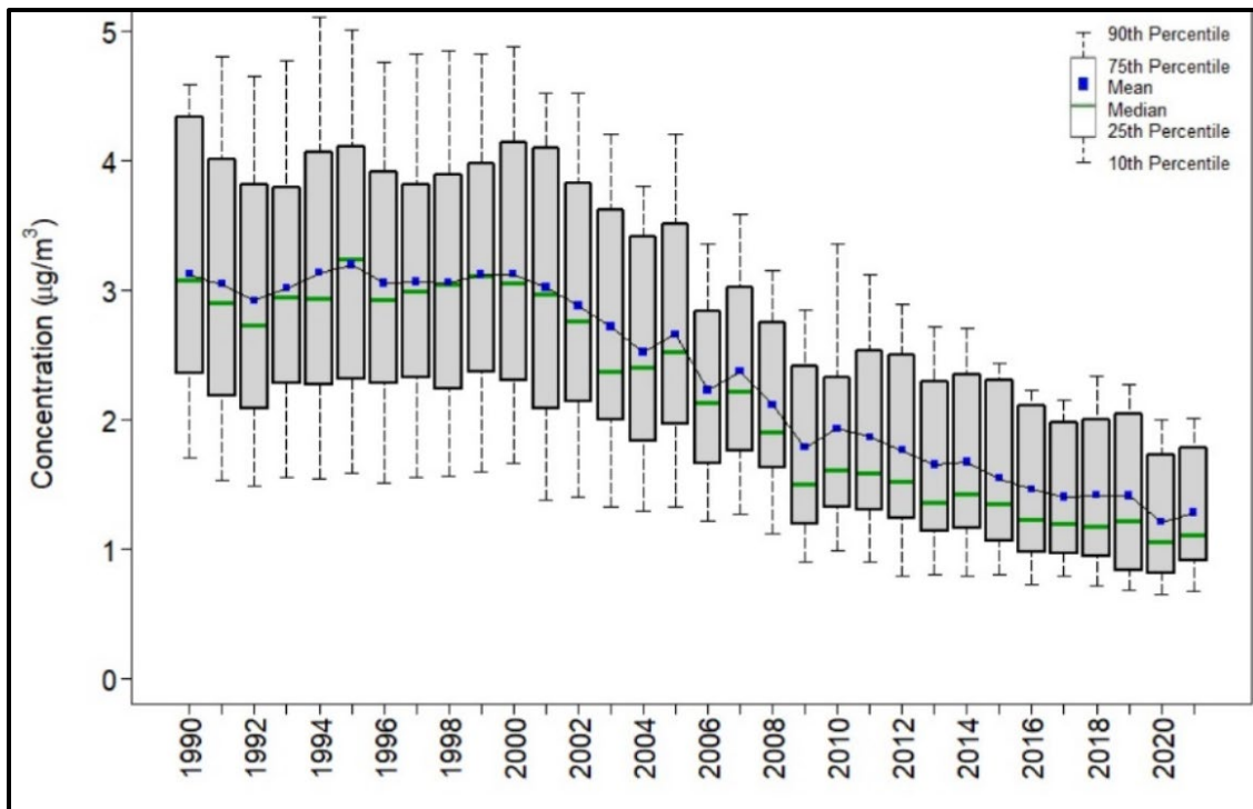
Figure 25. Trends in annual mean total nitrate concentrations – eastern reference sites.
