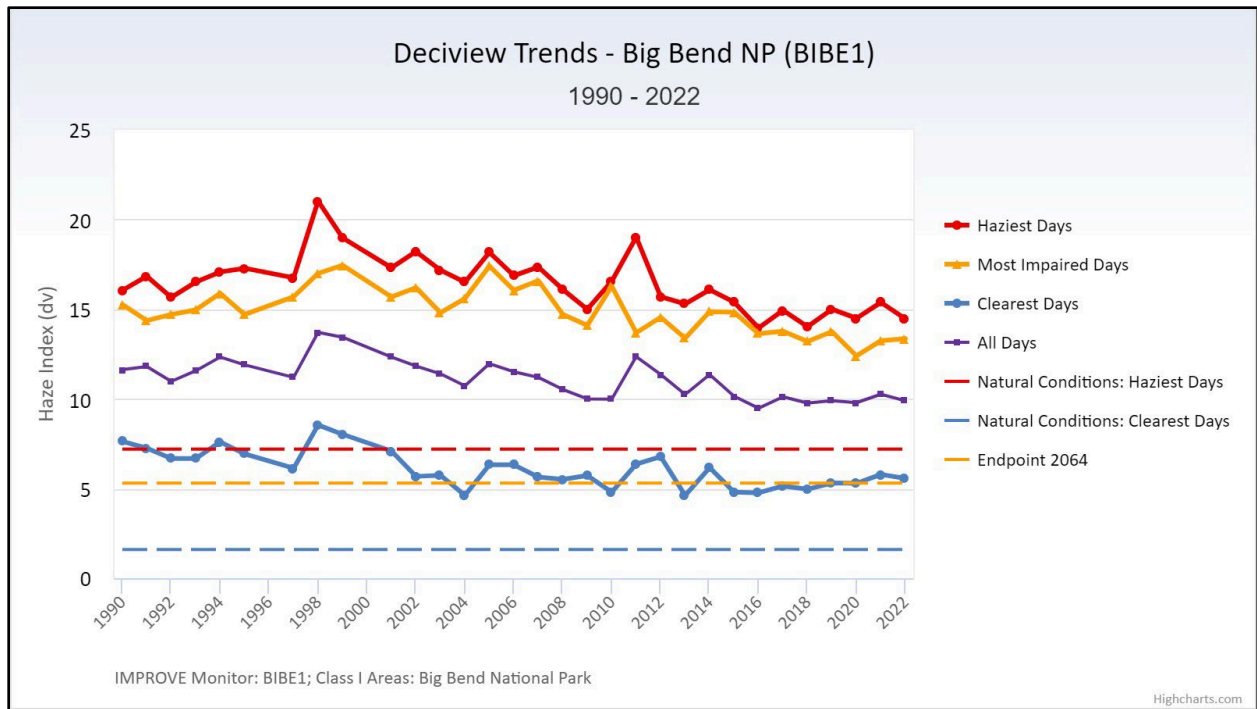
Figure 17. Visibility extinction trends for Big Bend National Park, Texas (FED CIRA 2024).
