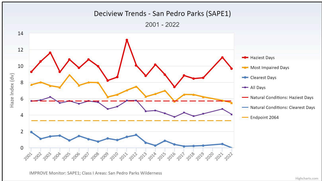
Figure 15. Visibility extinction trends for San Pedro Parks, New Mexico (FED CIRA 2024).
