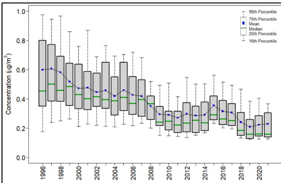
Figure 28. Trends in annual mean SO 2 concentrations – western reference sites.
