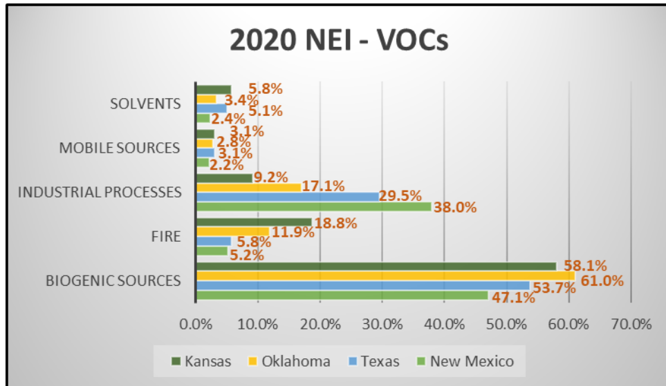
Figure 3. 2020 NEI – VOCs.
