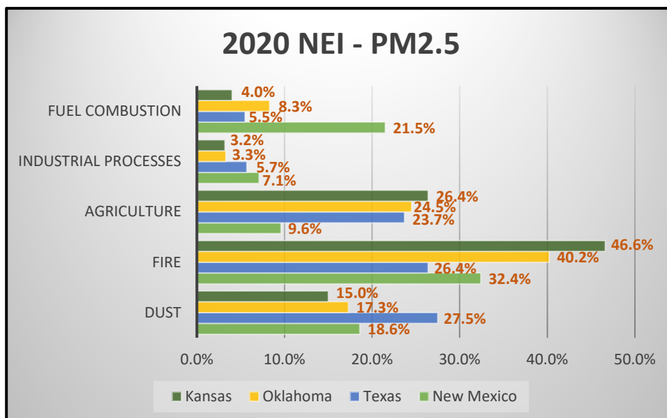
Figure 7. 2020 NEI - PM 2.5 .
