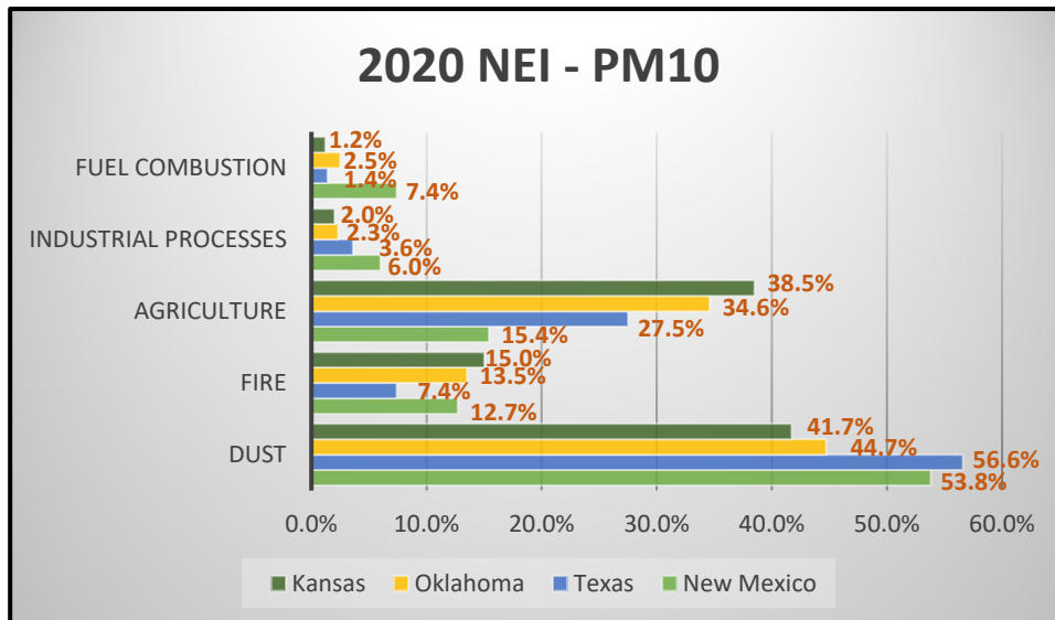
Figure 6. 2020 NEI - PM 10 .
