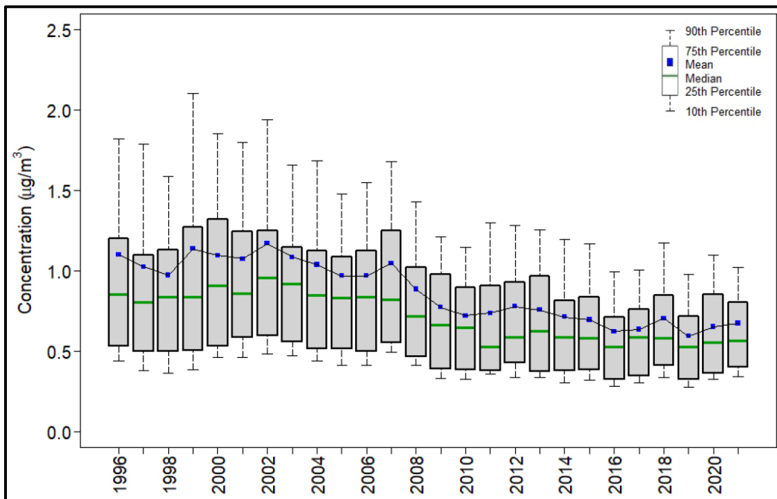
Figure 26. Trends in annual mean total nitrate concentrations – western reference sites.
