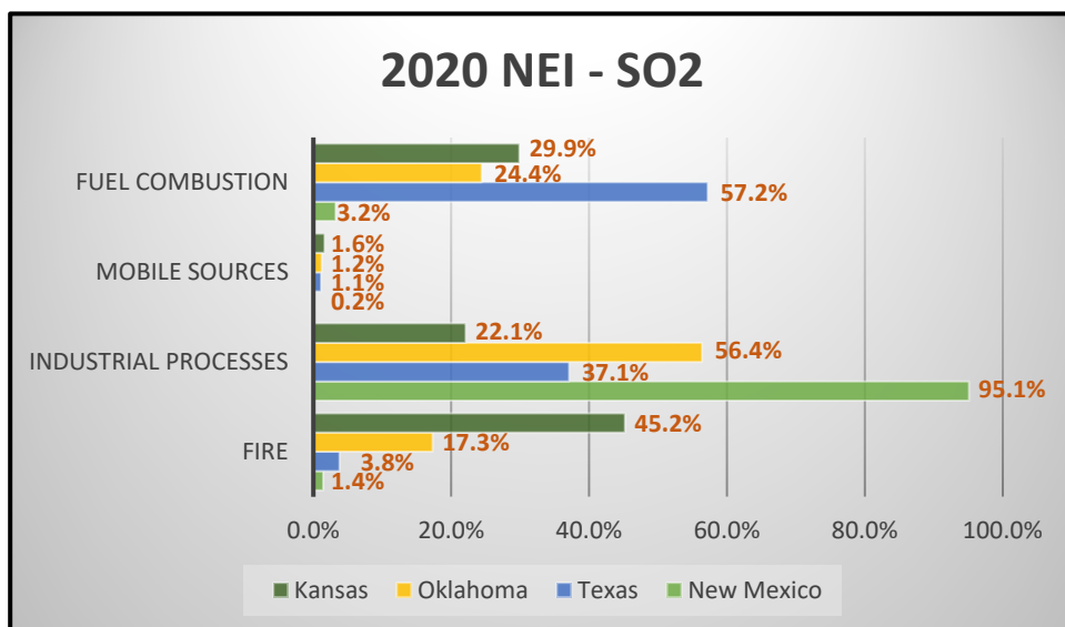
Figure 8. 2020 NEI - SO 2 .
