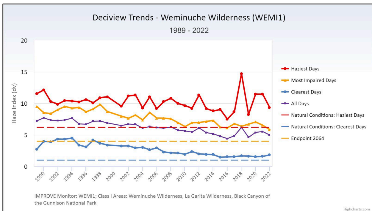
Figure 22. Visibility trends at Class I areas affected by sources in northwestern New Mexico – Weminuche Wilderness, Colorado (FED CIRA 2024).
