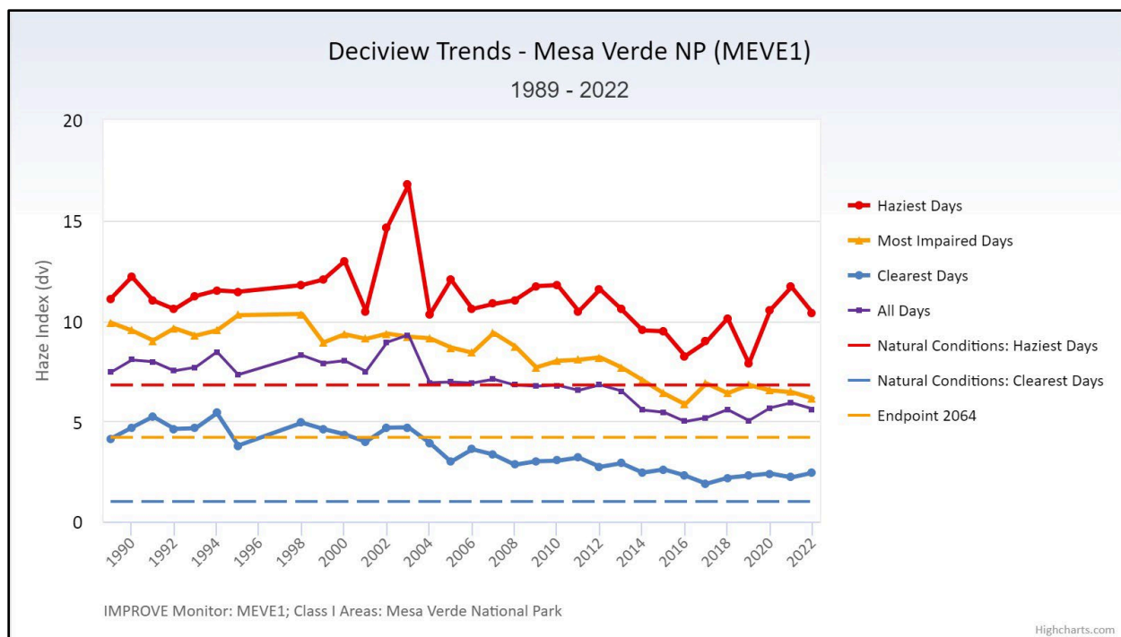
Figure 21. Visibility trends at Class I areas affected by sources in northwestern New Mexico – Mesa Verde National Park, Colorado (FED CIRA 2024).
