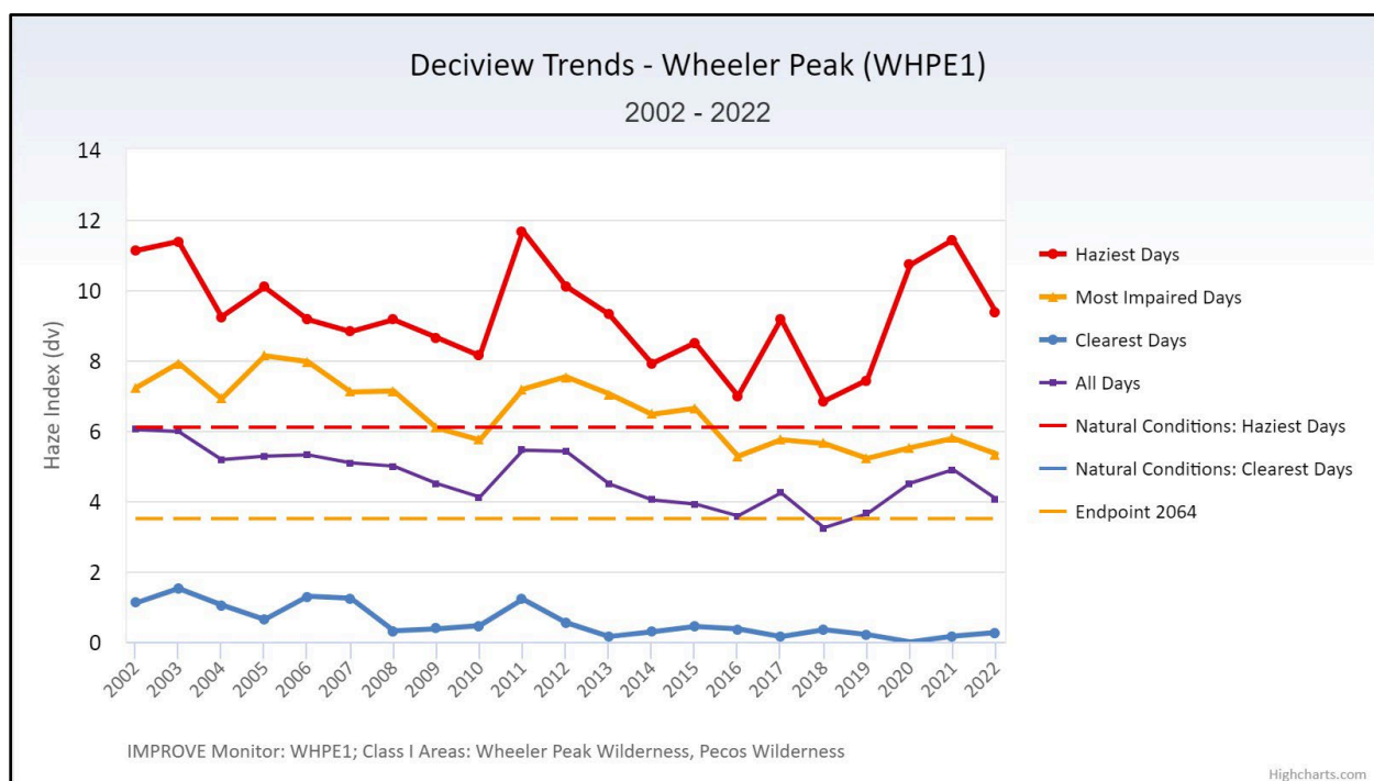
Figure 14. Visibility extinction trends for Wheeler Peak, New Mexico (FED CIRA 2024).
