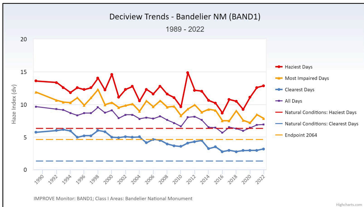
Figure 11. Visibility extinction trends for Bandelier National Monument, New Mexico (FED CIRA 2024).
