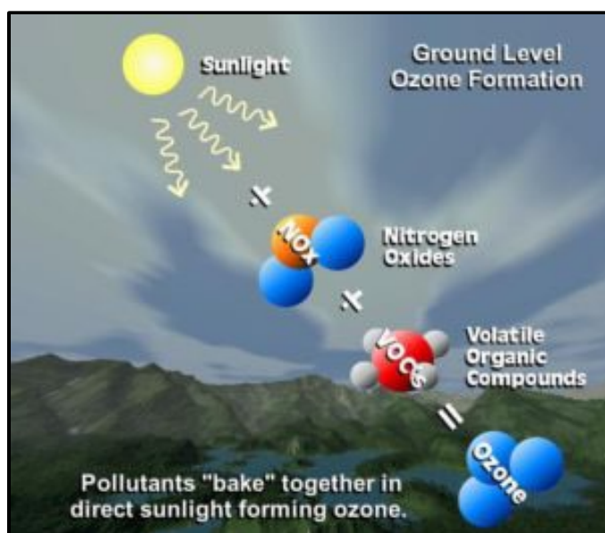
Figure 2. O_3 formation, courtesy of NASA.
