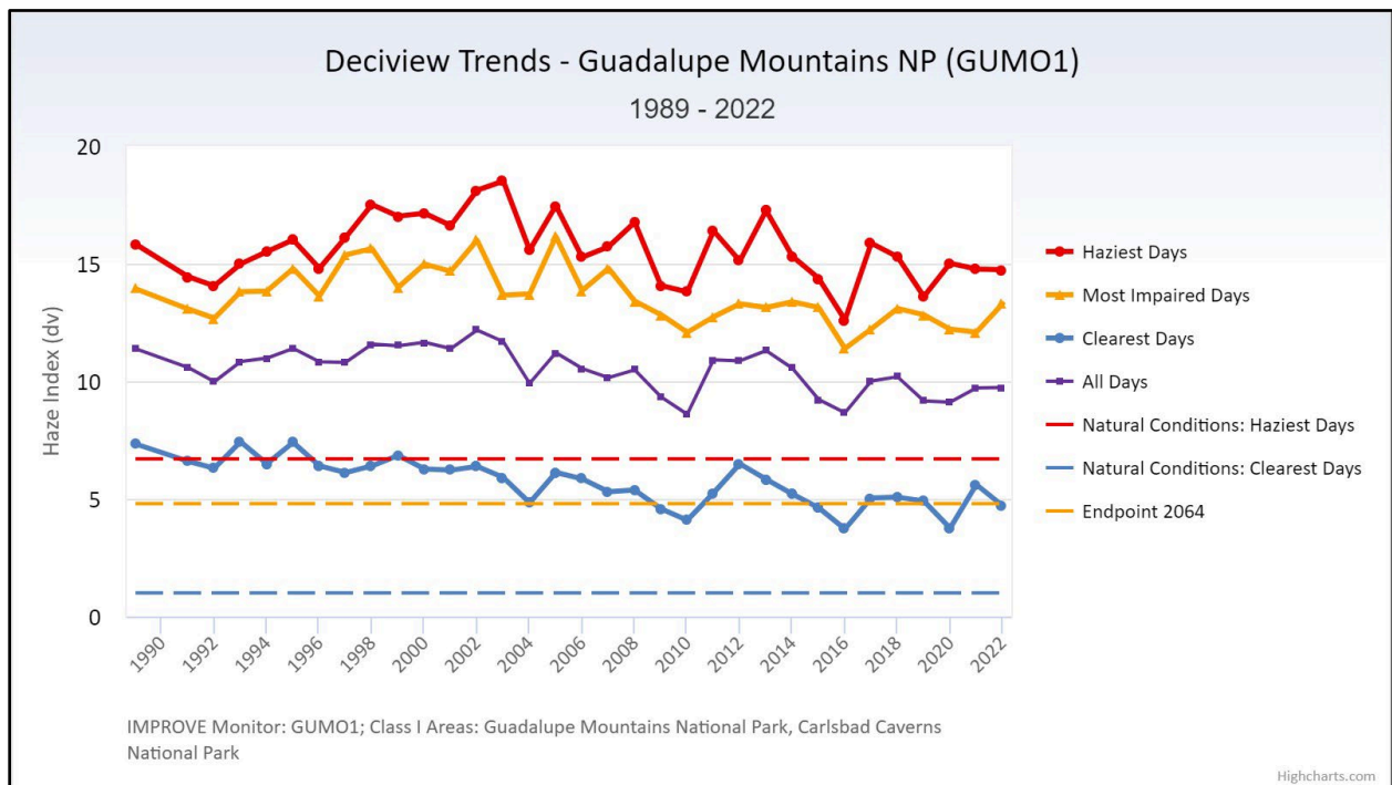
Figure 18. Visibility extinction trends for Guadalupe Mountains National Park, Texas (FED CIRA 2024).
