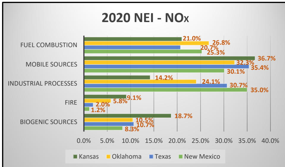
Figure 4. 2020 NEI – NO x .
