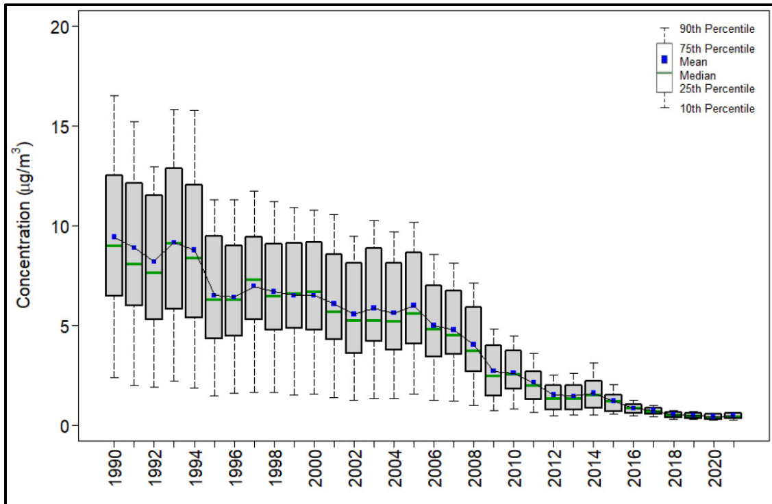
Figure 27. Trends in annual mean SO 2 concentrations – eastern reference sites.
