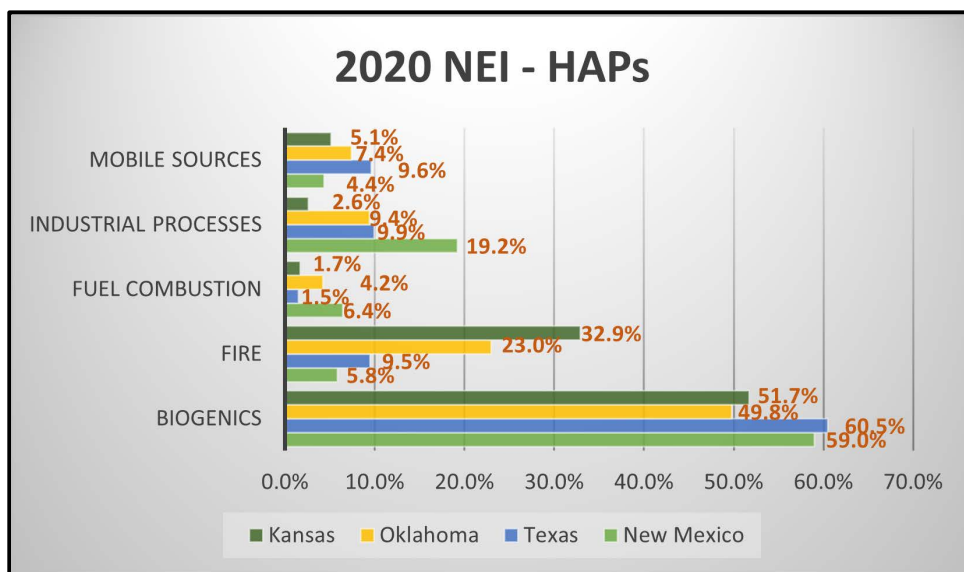
Figure 9. 2020 NEI - HAPs.
