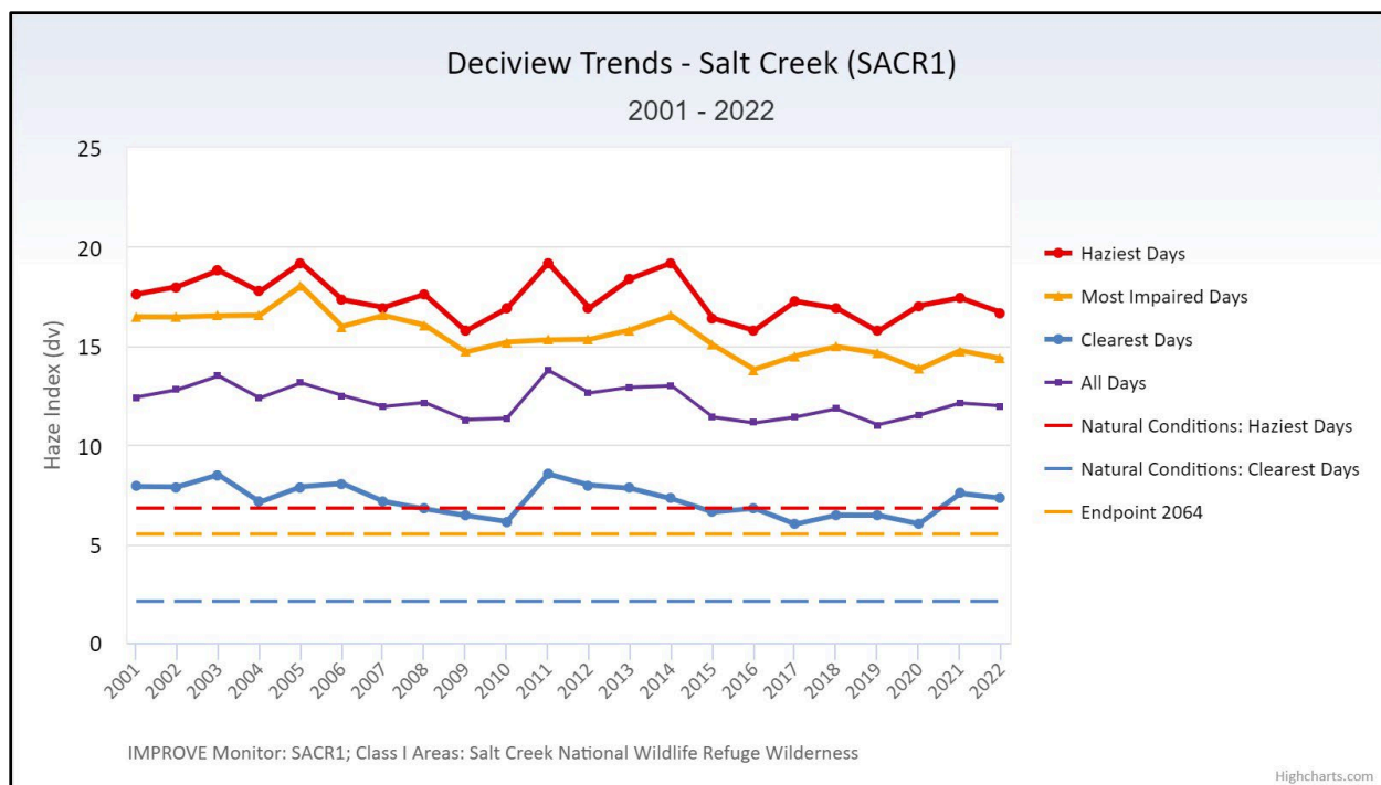
Figure 13. Visibility extinction trends for Salt Creek, New Mexico (FED CIRA 2024).
