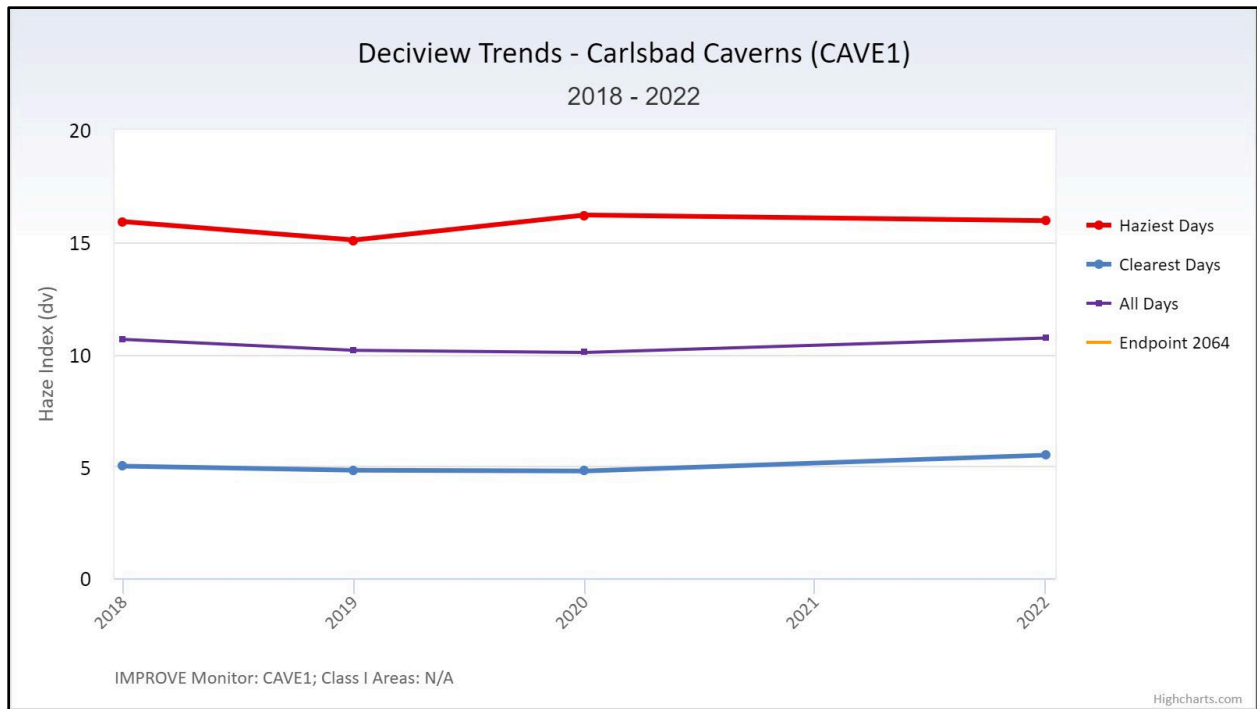
Figure 19. Visibility extinction trends for Carlsbad National Park, Texas (FED CIRA 2024).
