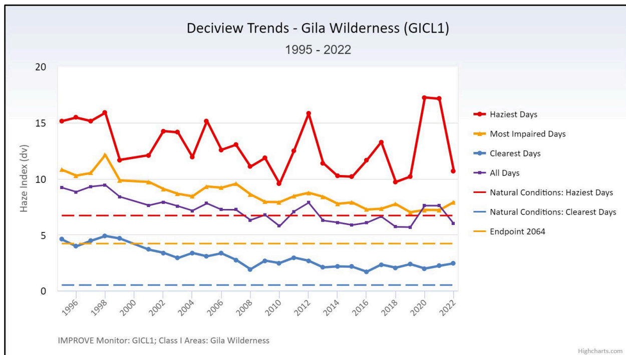
Figure 10. Visibility extinction trends for Gila Wilderness Area, New Mexico (FED Cooperative Institute for Research in the Atmosphere [CIRA] 2024).
