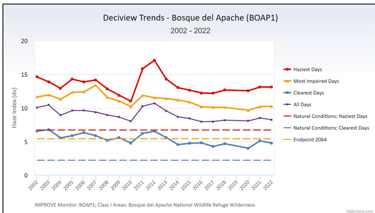
Figure 12. Visibility extinction trends for Bosque del Apache, New Mexico (FED CIRA 2024).
