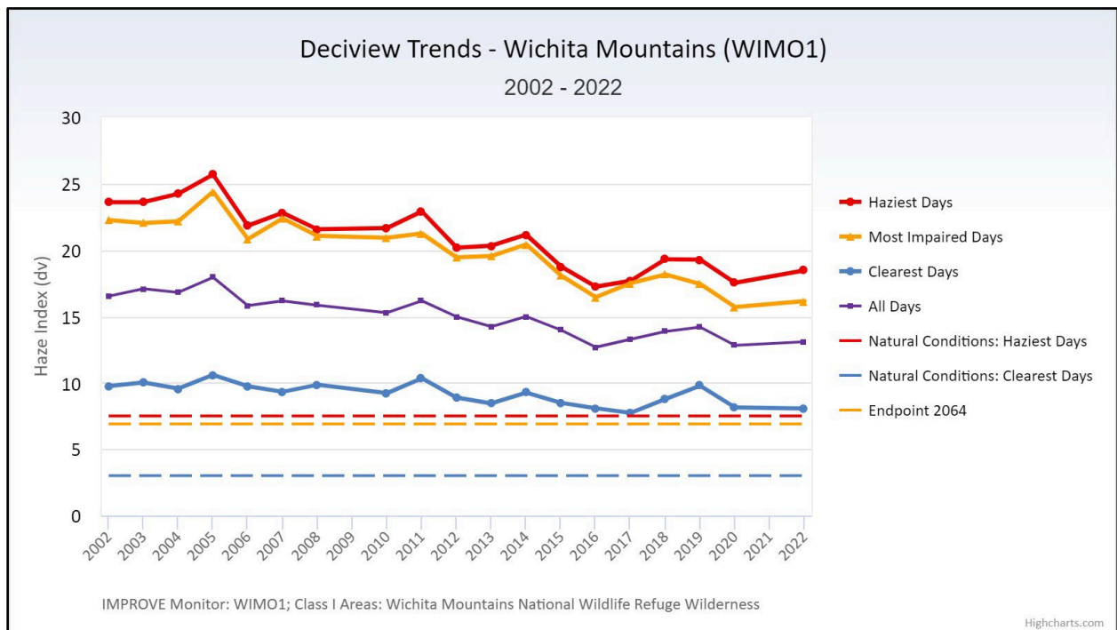
Figure 20. Visibility extinction trends for Wichita Mountains, Oklahoma (FED CIRA 2024).
