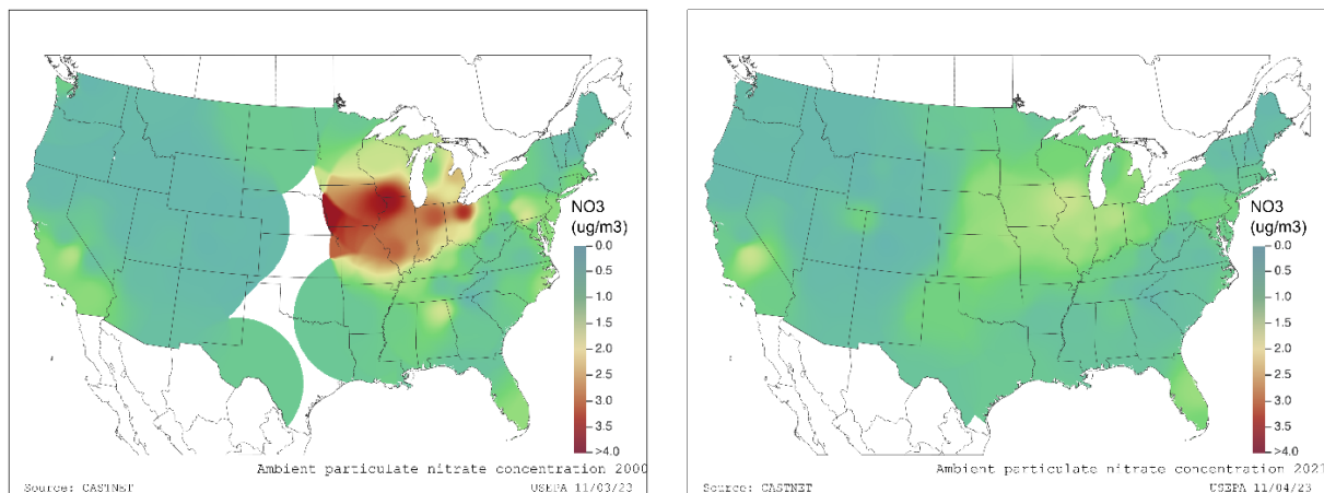
Figure 23. Particulate nitrate in 2000 (left) and 2021 (right).
